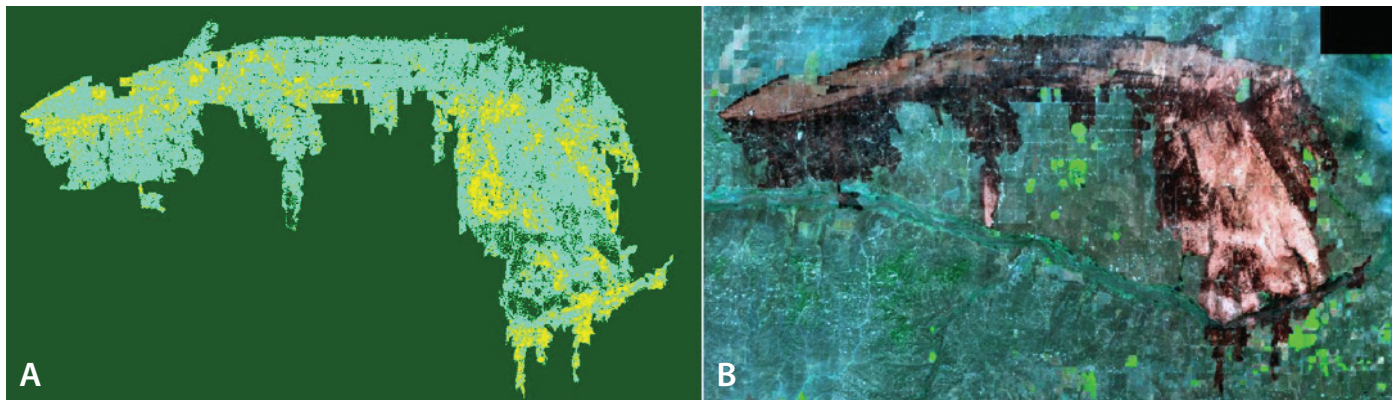
Figure 4. (A) Thresholded burn severity maps for Perryton wildfire in Ochiltree, Roberts, Hemphill and Lipscomb Counties, Texas that burned approximately 315,135 acres. Burn severity levels are: 1) dark green for unburned/very low (4,000 acres), 2) aquamarine for low (250,000 acres), 3) yellow for moderate (61,000 acres), and 4) red for high. (B) Aerial imagery of the Perryton area post-fire.
