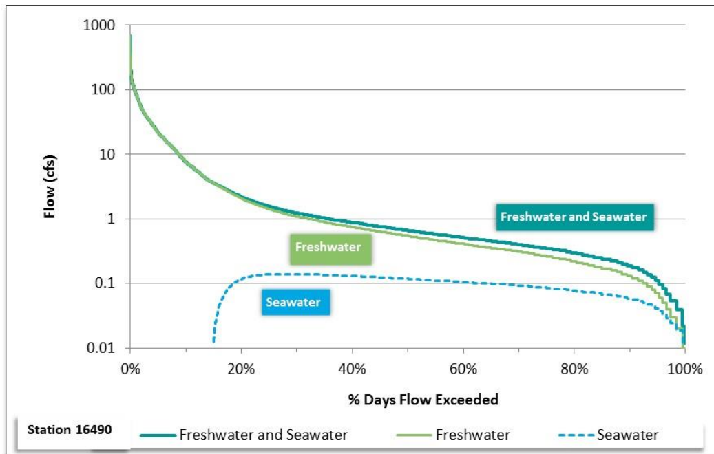
Figure 42. Modified FDC for station 16490, Marchand Bayou AU 2424C_01.
