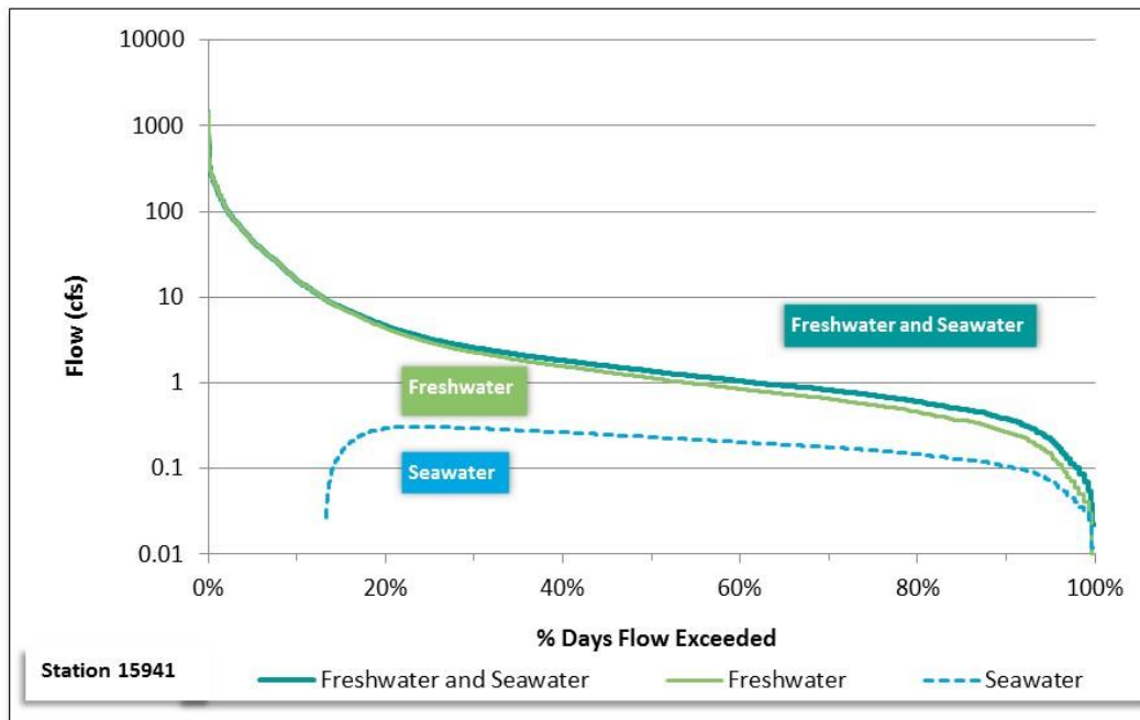
Figure 40. Modified FDC for station 15941, Highland Bayou AU 2424A_04.
