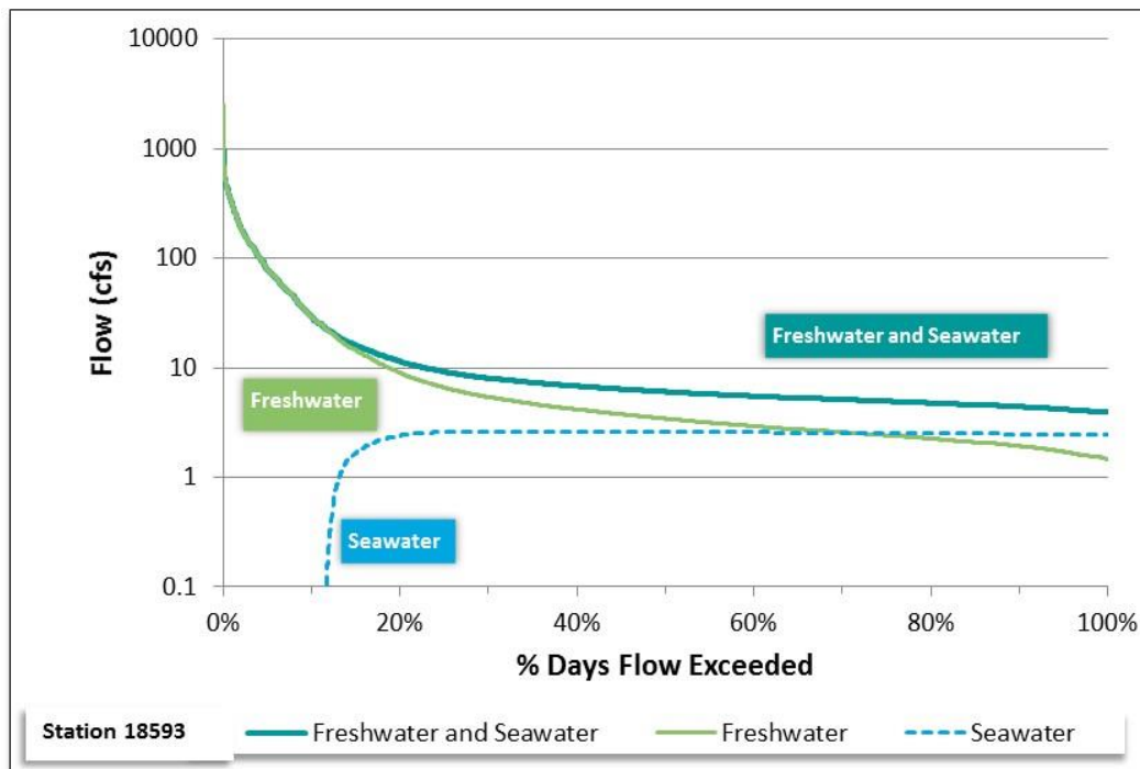
Figure 43. Modified FDC for station 18593, Highland Bayou Diversion Canal AU 2424G_01.
