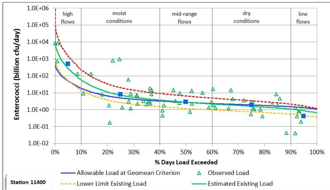
Figure 53. Modified LDC for station 11400, Moses Bayou AU 2431A_01
