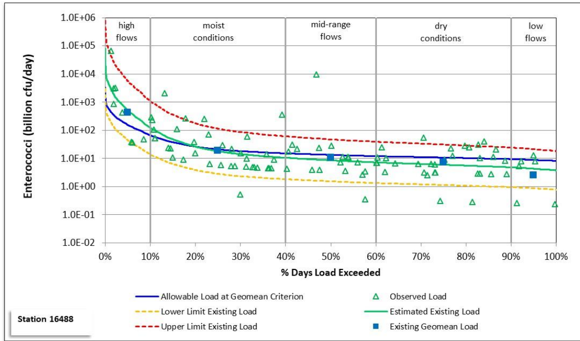
Figure 46. Modified LDC for station 16488, Highland Bayou AU 2424A_01.
