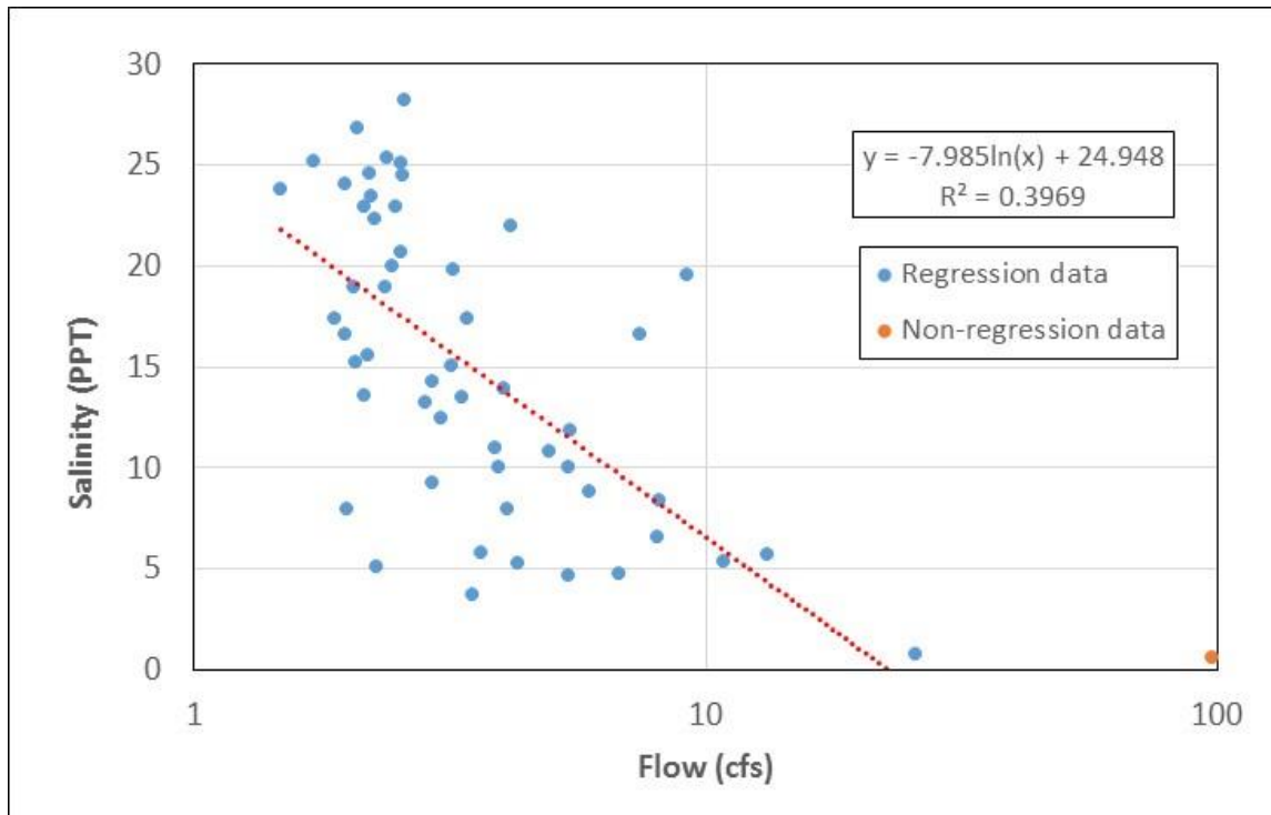
Figure 14 Scatter plot of salinity and estimated daily streamflow for station 18593, Highland Bayou Diversion Canal AU 2424G_01. This graphical depiction of the salinity to flow relationship is characteristic of those developed for all waterbodies in the project.
