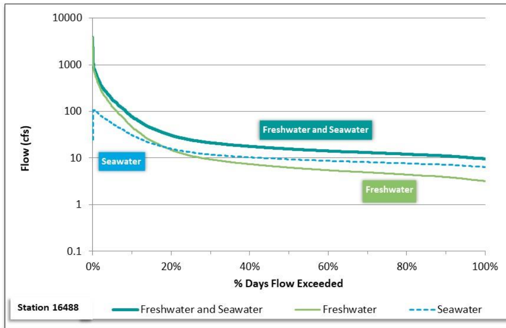
Figure 15. Modified FDC for station 16488, Highland Bayou AU 2424A_01
