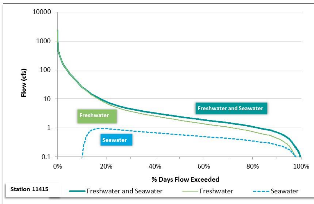
Figure 39. Modified FDC for station 11415, Highland Bayou AU 2424A_03.
