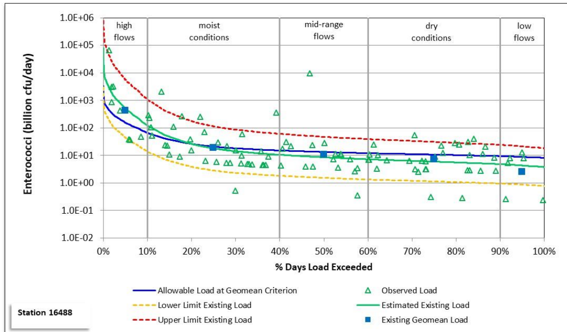
Figure 17. Modified LDC for station 16488, Highland Bayou AU 2424A_01, this station is nearest the mouth of Highland Bayou
