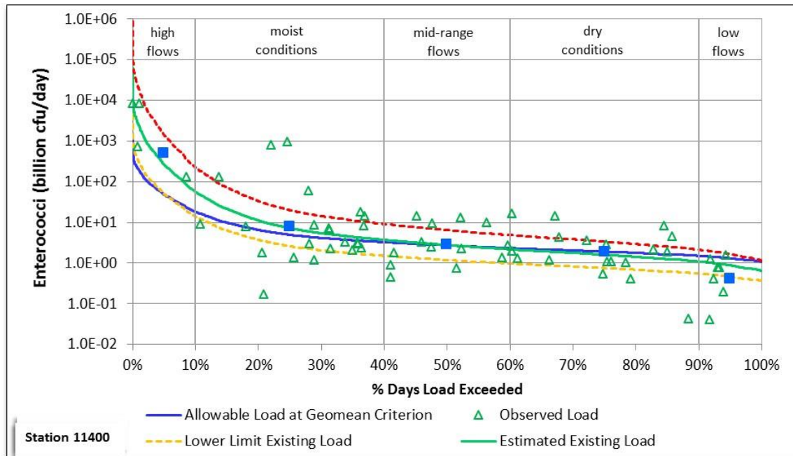
Figure 20. Modified LDC for station 11400, Moses Bayou AU 2431A_01
