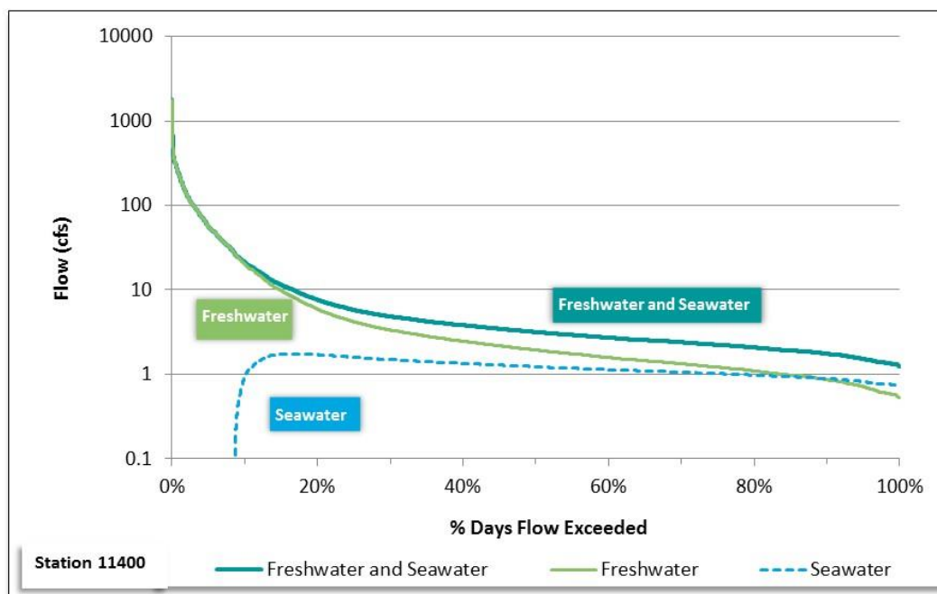
Figure 44. Modified FDC for station 11400, Moses Bayou AU 2431A_01
