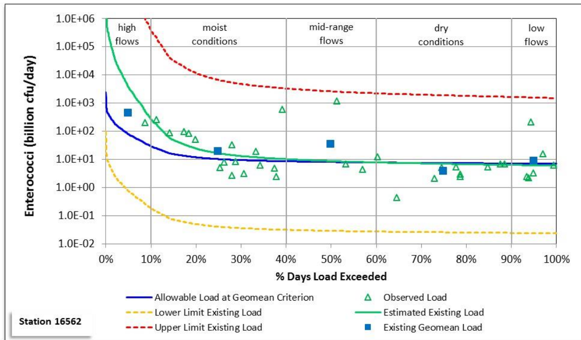
Figure 47. Modified LDC for station 16562, Highland Bayou AU 2424A_02.
