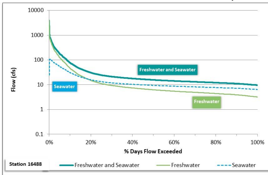
Figure 37. Modified FDC for station 16488, Highland Bayou AU 2424A_01.
