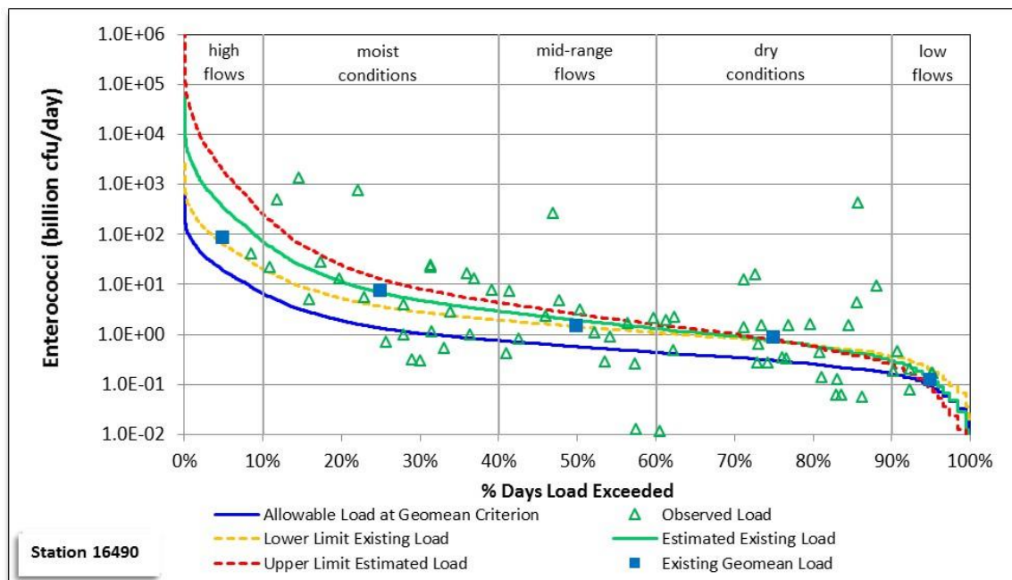
Figure 51. Modified LDC for station 16490, Marchand Bayou AU 2424C_01.
