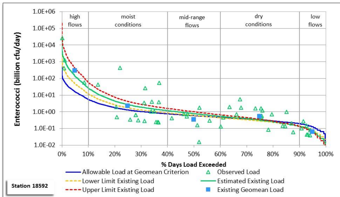
Figure 21. Modified LDC for station 18592, Unnamed Tributary of Moses Lake AU 2431C_01
