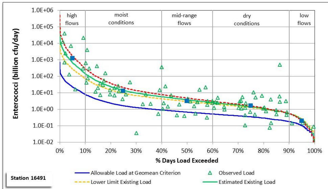
Figure 50. Modified LDC for station 16491, Highland Bayou AU 2424A_05.
