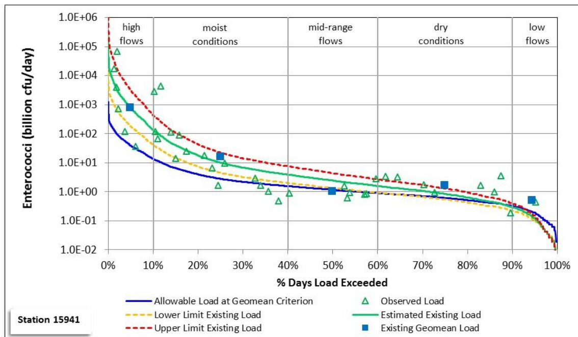
Figure 49. Modified LDC for station 15941, Highland Bayou AU 2424A_04.
