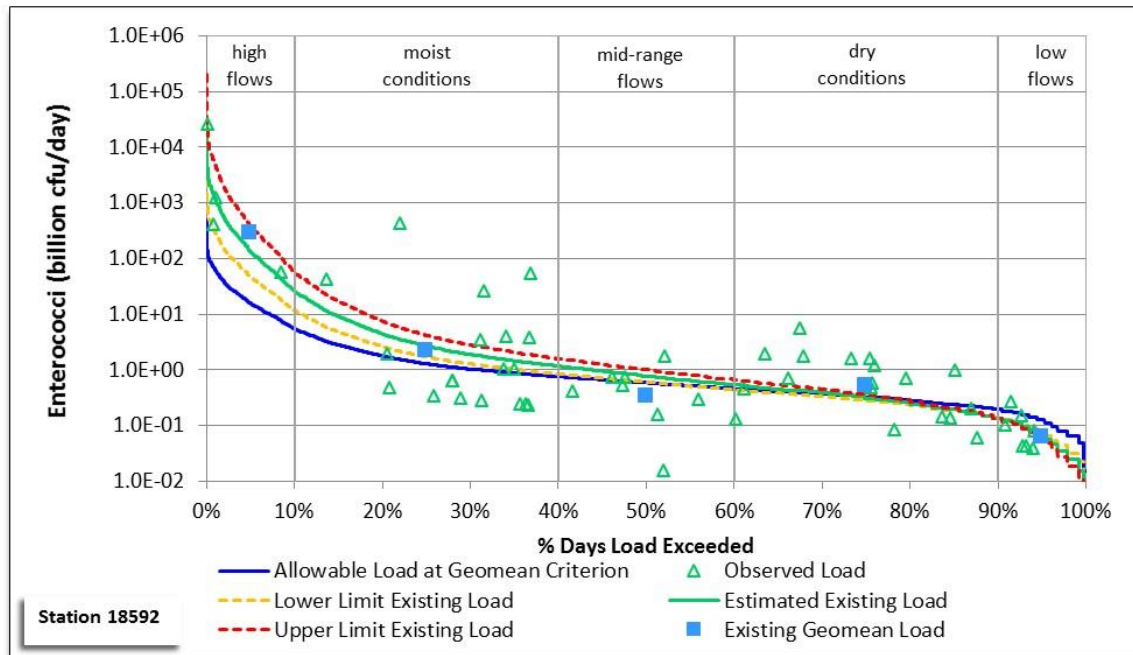
Figure 54. Modified LDC for station 18592, Unnamed Tributary of Moses Lake AU 2431C_01
