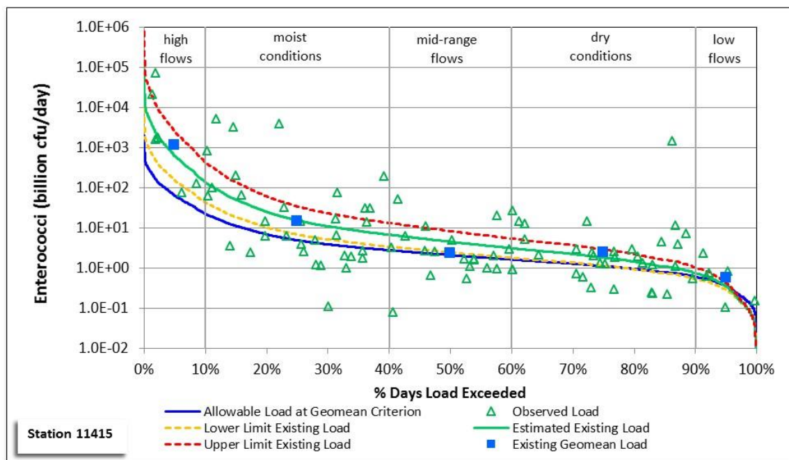
Figure 48. Modified LDC for station 11415, Highland Bayou AU 2424A_03.
