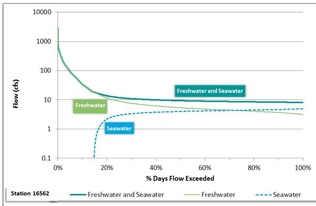
Figure 38. Modified FDC for station 16562, Highland Bayou AU 2424A_02.
