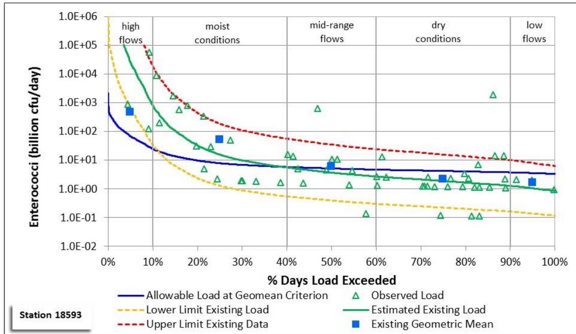
Figure 52. Modified LDC for station 18593, Highland Bayou Diversion Canal AU 2424G_01.
