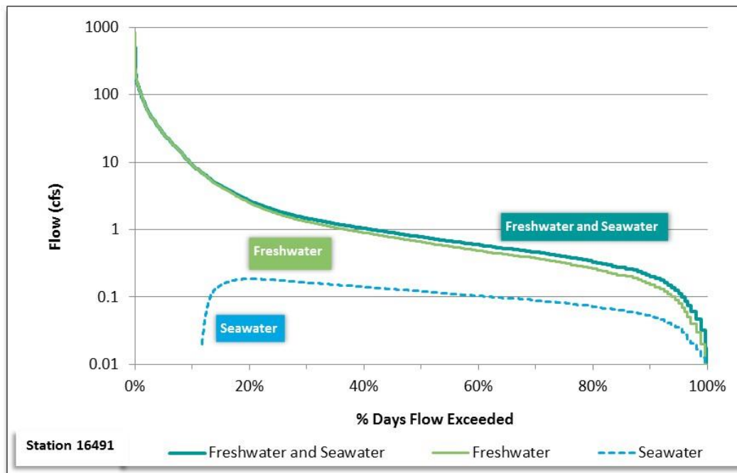
Figure 41. Modified FDC for station 16491, Highland Bayou AU 2424A_05.
