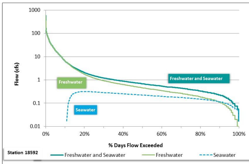
Figure 45. Modified FDC for station 18592, Unnamed Tributary of Moses Lake AU 2431C_01
