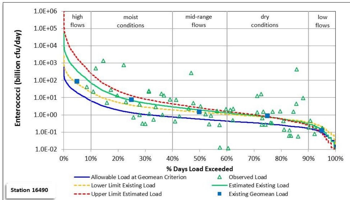
Figure 18. Modified LDC for station 16490, Marchand Bayou AU 2424C_01
