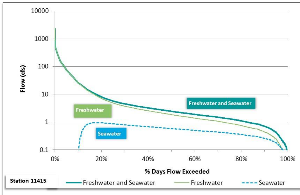
Figure 16. Modified FDC for station 11415, Highland Bayou AU 2424A_03
