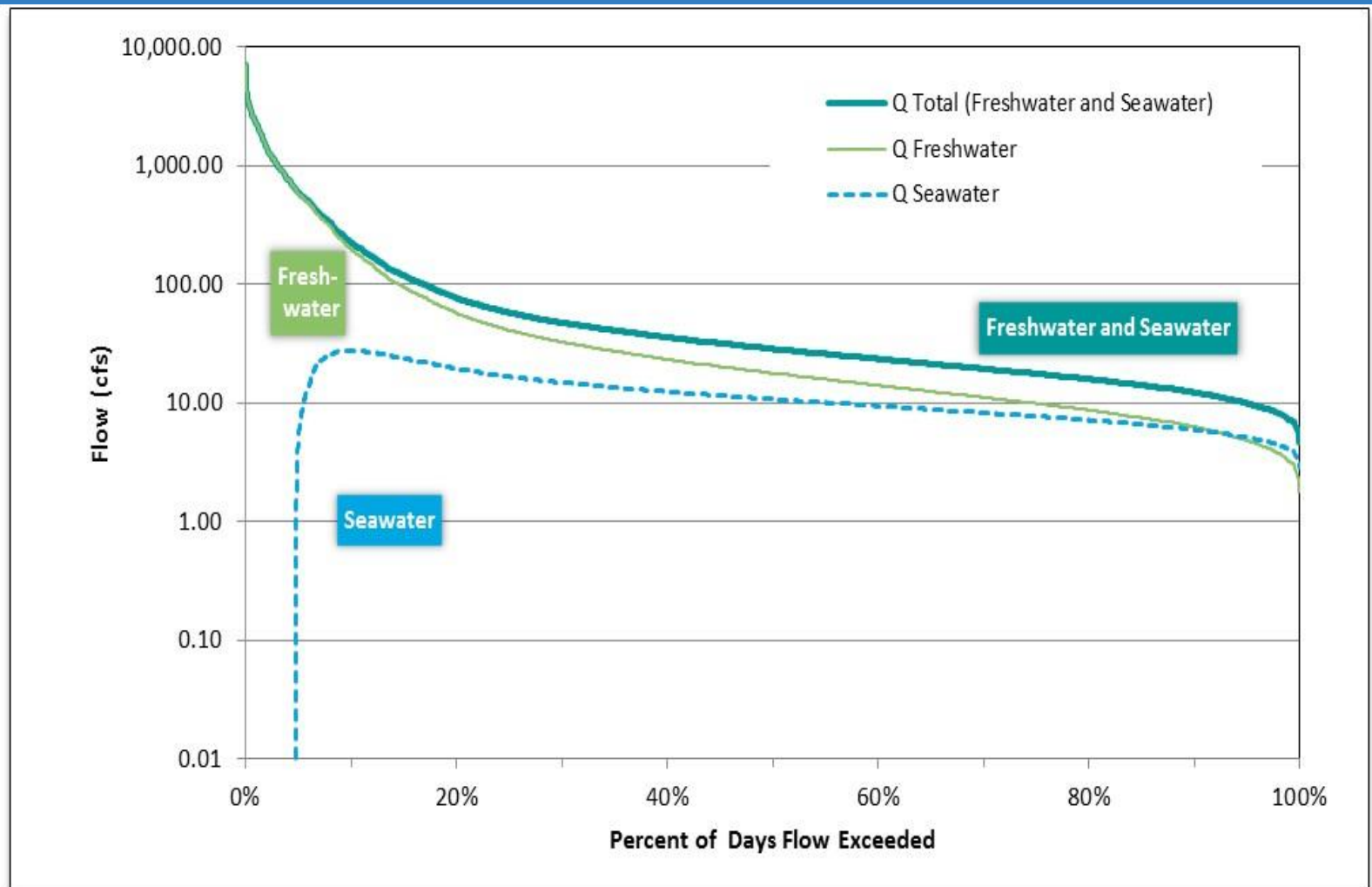
FDC Dickinson Bayou Tidal Station 11455 showing freshwater and seawater components of the flow.
