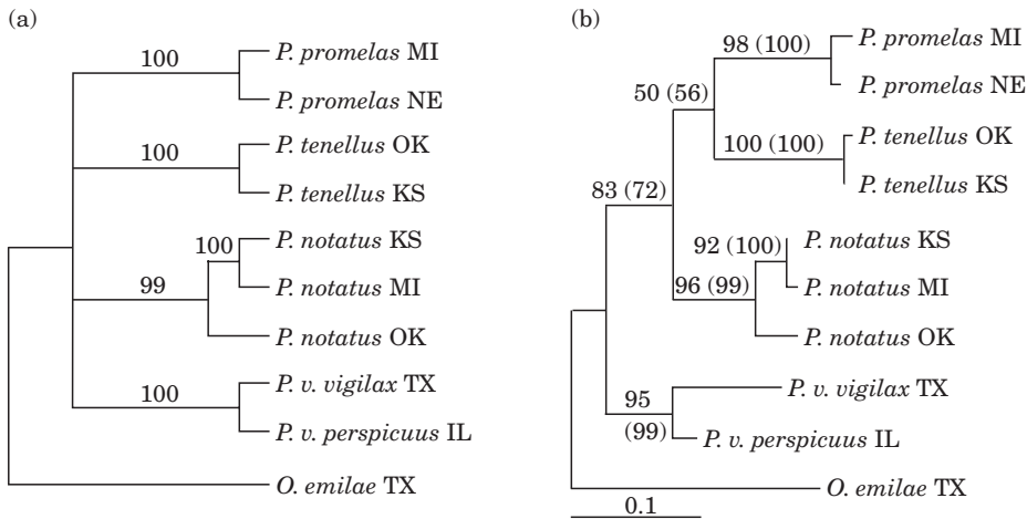
FIG. 1. Estimates of the Pimephales phylogeny derived from analysis of mitochondrially-encoded ND4-ND4L sequences. (a) Strict consensus of four equally parsimonious (MP) trees (length=244 steps). Numbers at nodes are bootstrap proportions. (b) Tree topology derived from both maximum-likelihood (ML) analysis ( \ell = -1728.04 ) under the GTR substitution matrix (Yang, 1994a) in combination with a discrete Gamma (d \Gamma ) model of among sites rate variation (Yang, 1994b), and minimum-evolution (ME) analysis (tree score=0.4936) of LogDet distances (Lockhart et al. , 1994). Branch lengths are proportional to mean number of nucleotide substitutions per site, as inferred under the GTR+d \Gamma model. Numbers at nodes are bootstrap proportions for ML and, in parentheses, ME. IL, Illinois; KS, Kansas; MI, Michigan; NE, Nebraska; OK, Oklahoma; TX, Texas.
