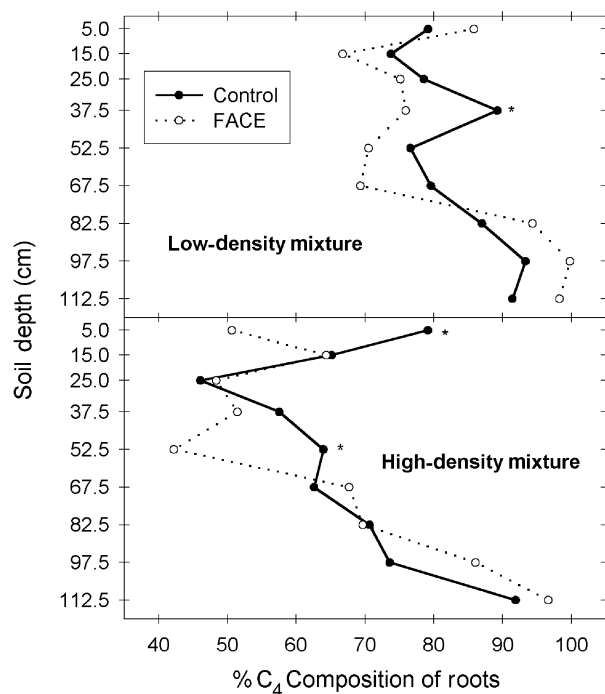
Fig. 2 Mean ( n=2 ) % C_4 composition of roots, derived using \delta^{13}C values of roots and mass balance equation (See Methods), by depth from 4.1 cm \times 120 cm soil cores beneath plants within 1-m rows of low-density (5 plants of each species m^{-1} row length) and high-density (10 plants of each species m^{-1} row length) mixtures of sorghum and cotton plants on 29 August following exposure to two CO_2 treatments (daytime CO_2 concentrations: FACE, 566 \mu mol\ mol^{-1} ; Control, 373 \mu mol\ mol^{-1} ) and two soil water treatments (Wet and Dry).
