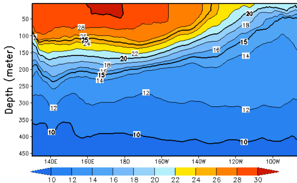
Equatorial T Penatd Mean ( ^{\circ}\text{C} ), Aug 11 2019
