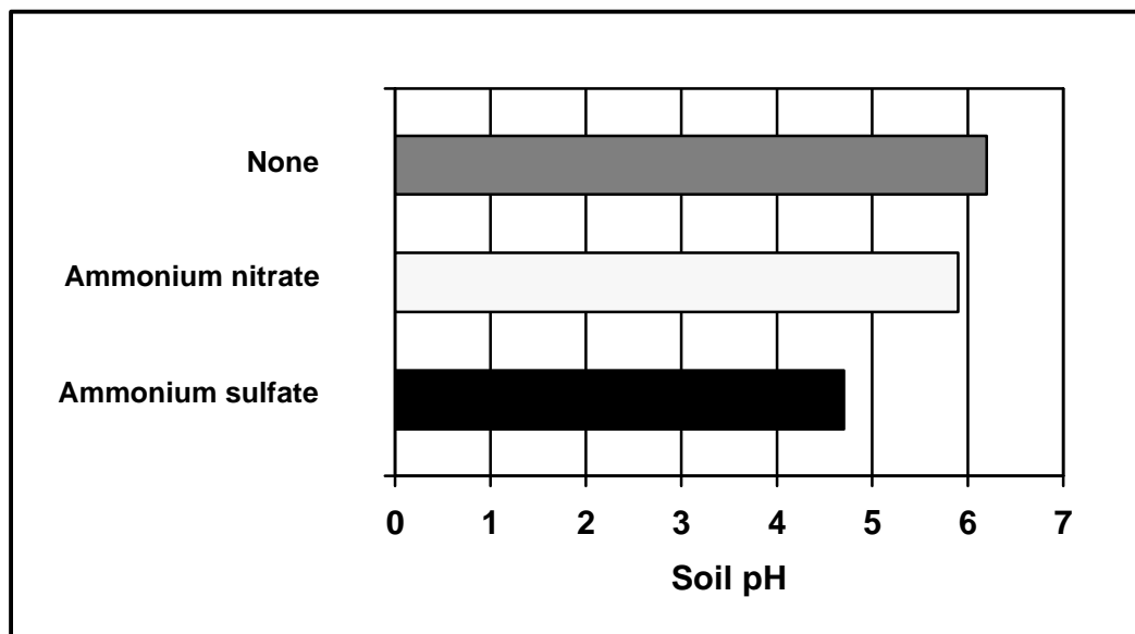
Figure 1. Effect on soil pH of different N fertilizer sources after three years. TAMU-Overtton
