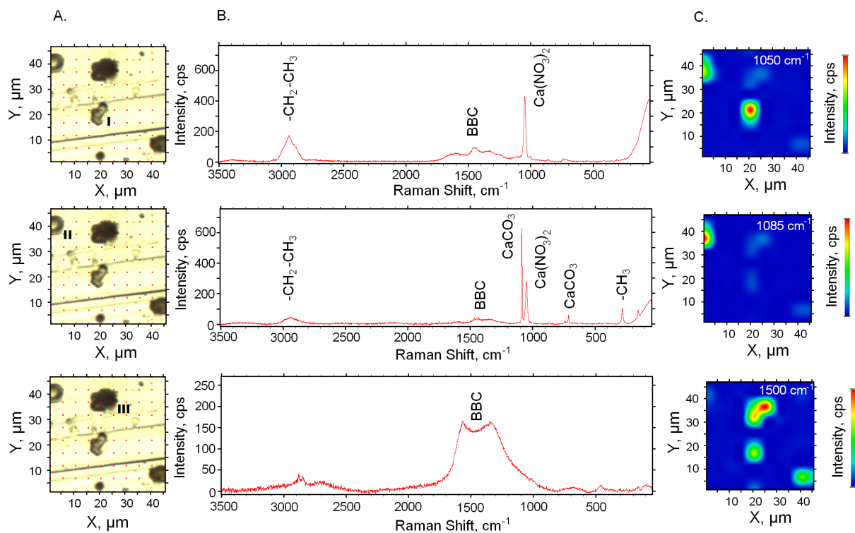
Fig. 7. In (A), microscopic image of Particles I, II, and III collected from upwind location July 22 at ~9:00 p.m. In (B), the full Raman spectra of Particle I, II, and III are shown. In (C), spectral maps of major components of the particles are shown including Ca (NO 3 ) 2 at 1050 cm -1 , CaCO 3 at 1085 cm -1 , and black or brown carbon (BBC) at ~1500 cm -1 .
