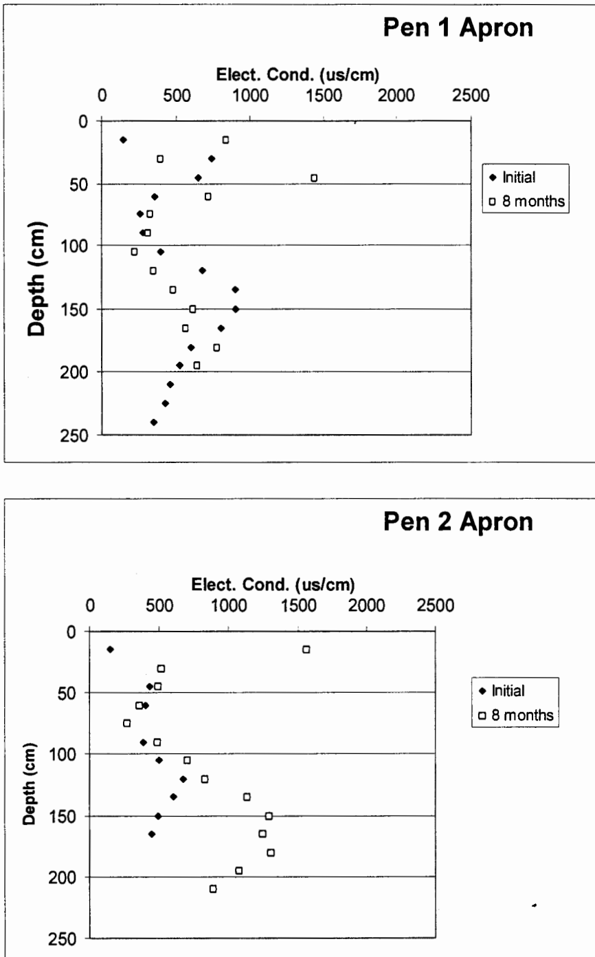
Figure 2. Graphs of soil electrical conductivity with depth for apron area.
